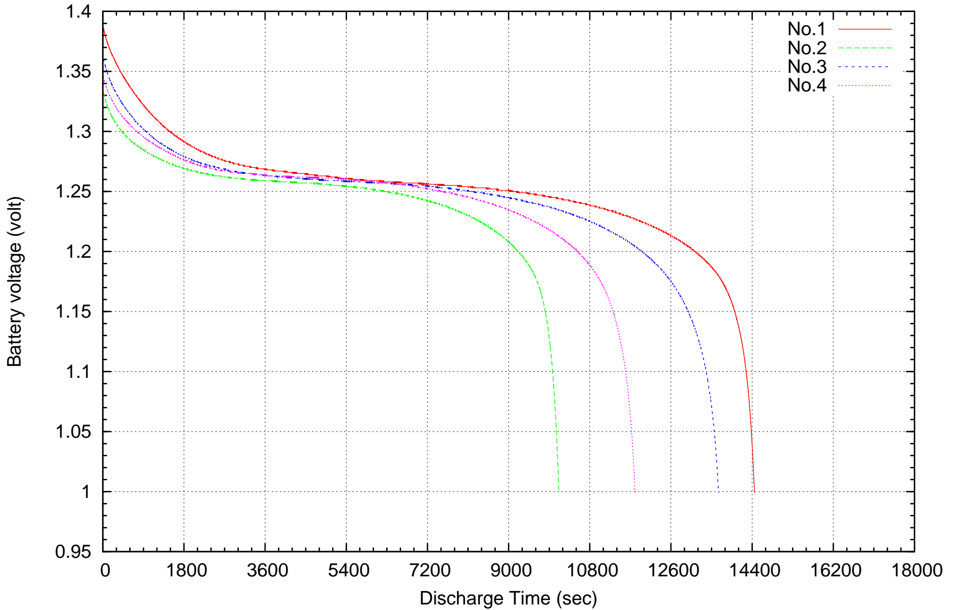
GP-ecototal-AAA MR900AAA special sale at Akizuki Yashio, 0.2C discharge battery voltage vs discharge time
