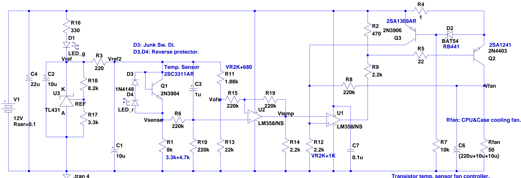
Transistor temp. sensor fan controller. 2010.11.30 FTechWorks.
